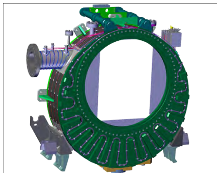
Figure 8: General views of HNB2 VVPSS Box (interface DN300)
