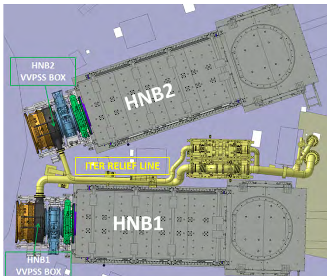
Figure 2: Top view of VVPSS line in the NB Cell configuration PFPO1
