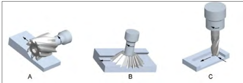
Figure 17: Machining method for Metallic seal groove
