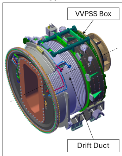
Figure 13 : Batch VVPSS Box Welded to the Drift Duct
