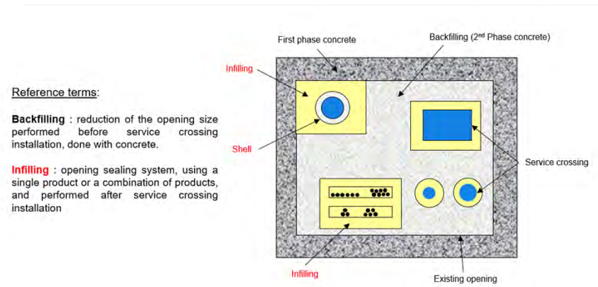
Schematic of wall sealing / infilling components
