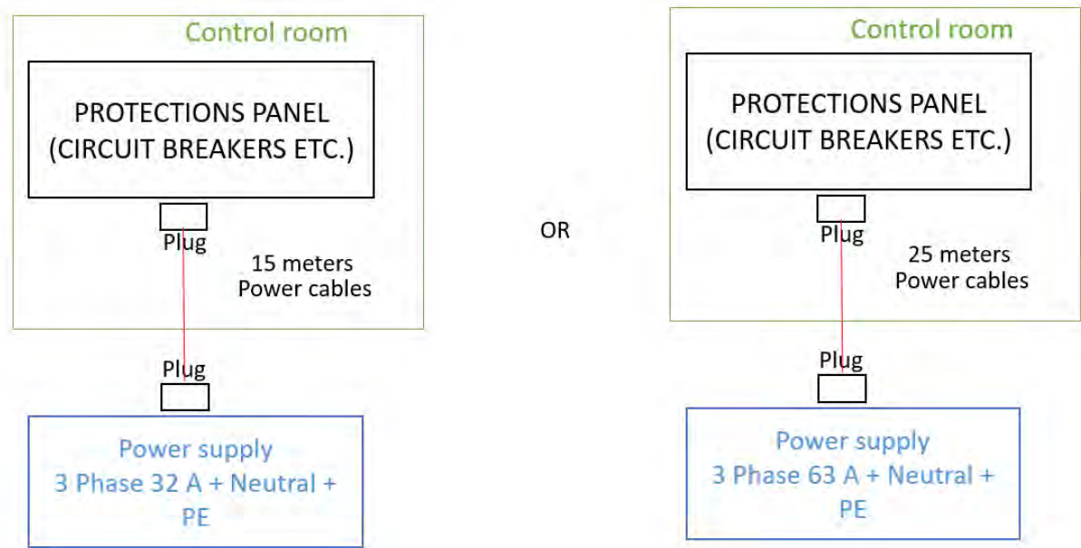
Figure 8 Interface Protection panel – Power supply
