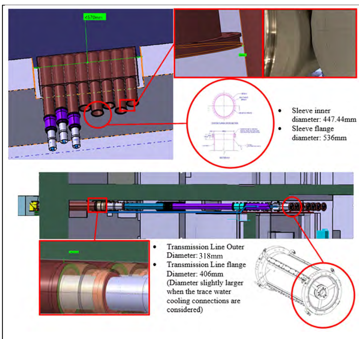
Figure 5: South Wall Penetration Dimensions
