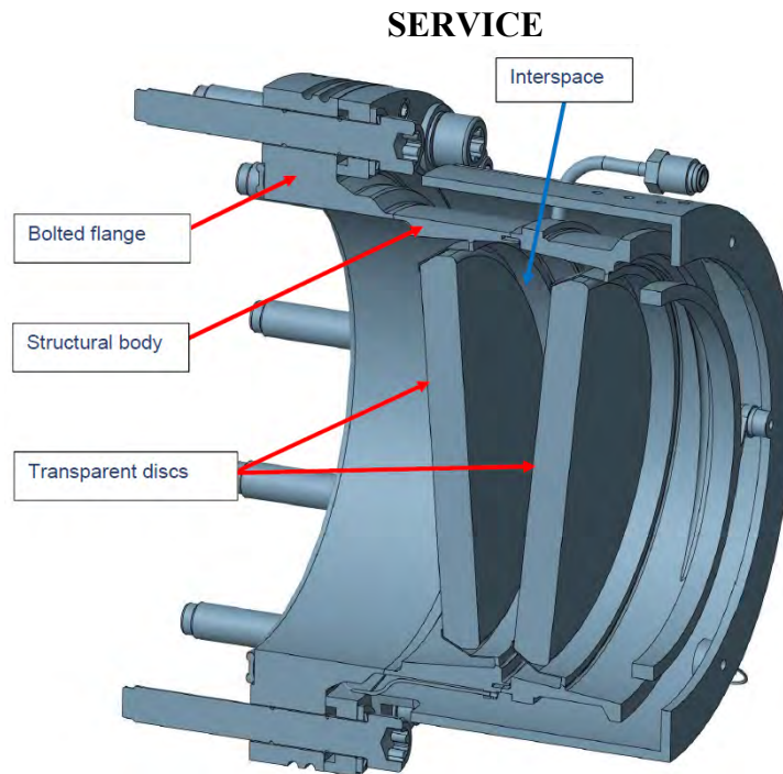
Figure 2: Section of Window Assembly
